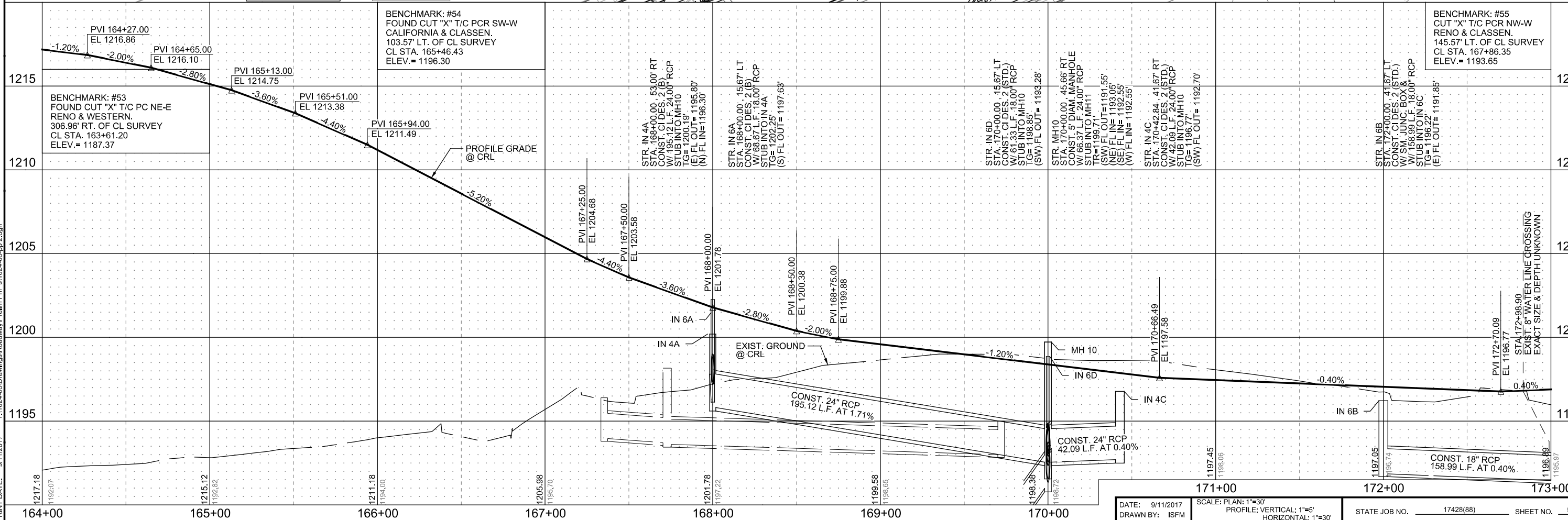
PLAN AND PROFILE - OKLAHOMA CITY BOULEVARD - OKLAHOMA COUNTY
